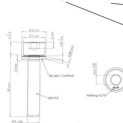
M4x20 M4x20 CAPSULE DN-F12 Marking A2-70
